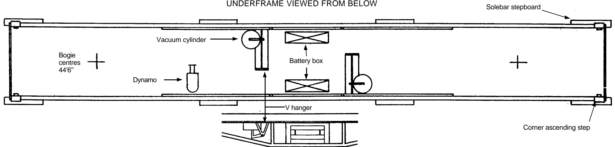
UNDERFRAME VIEWED FROM BELOW
