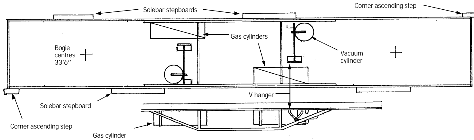
UNDERFRAME VIEWED FROM BELOW
