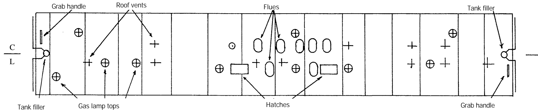
ROOF AND INTERIOR PLANS VIEWED FROM ABOVE
